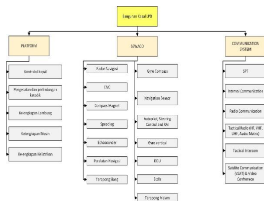
Gambar 2. WBS Kapal Landing Platform Dock (LPD)
